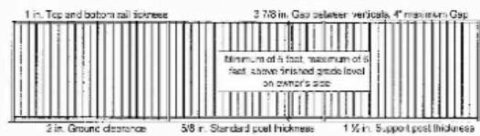
Elevation B: Wrought Iron Party Fence
